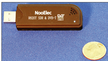
An RTL-SDR dongle receiver.
