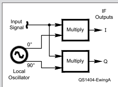
Figure A — In-phase and quadrature IFs.
